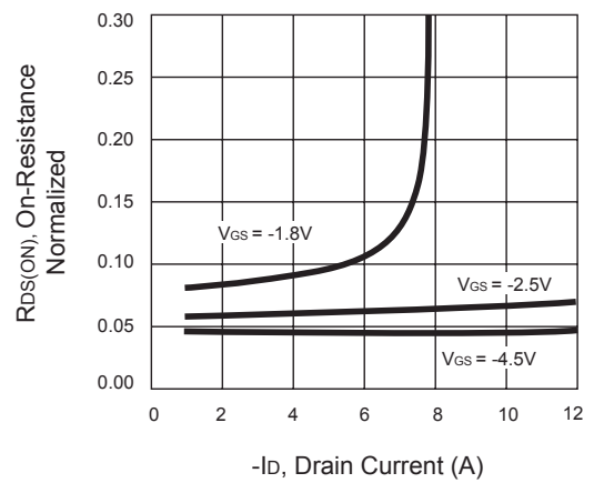
Figure 6. On-Resistance Variation with Drain Current
